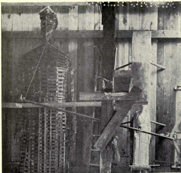
FIG. 42—BUILDING FRAMEWORK FOR CLAY MODEL 16' HIGH FOR CONCRETE STATUES, USING PANTOGRAPH IN CONNECTION WITH \frac{1}{4} -SIZE MODEL
